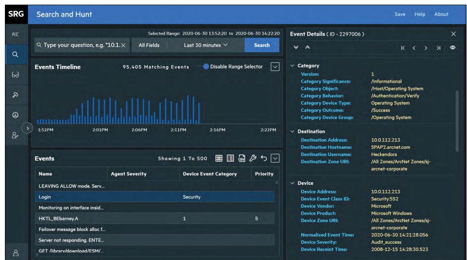
Figure 3. ArcSight Recon
