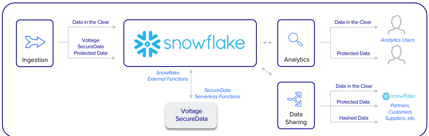
Figure 1. Voltage SecureData integration with Snowflake for Secure Analytics and Data Sharing
