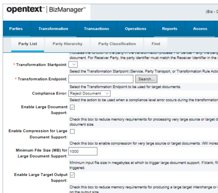
Enable unlimited files sizes for data translation
